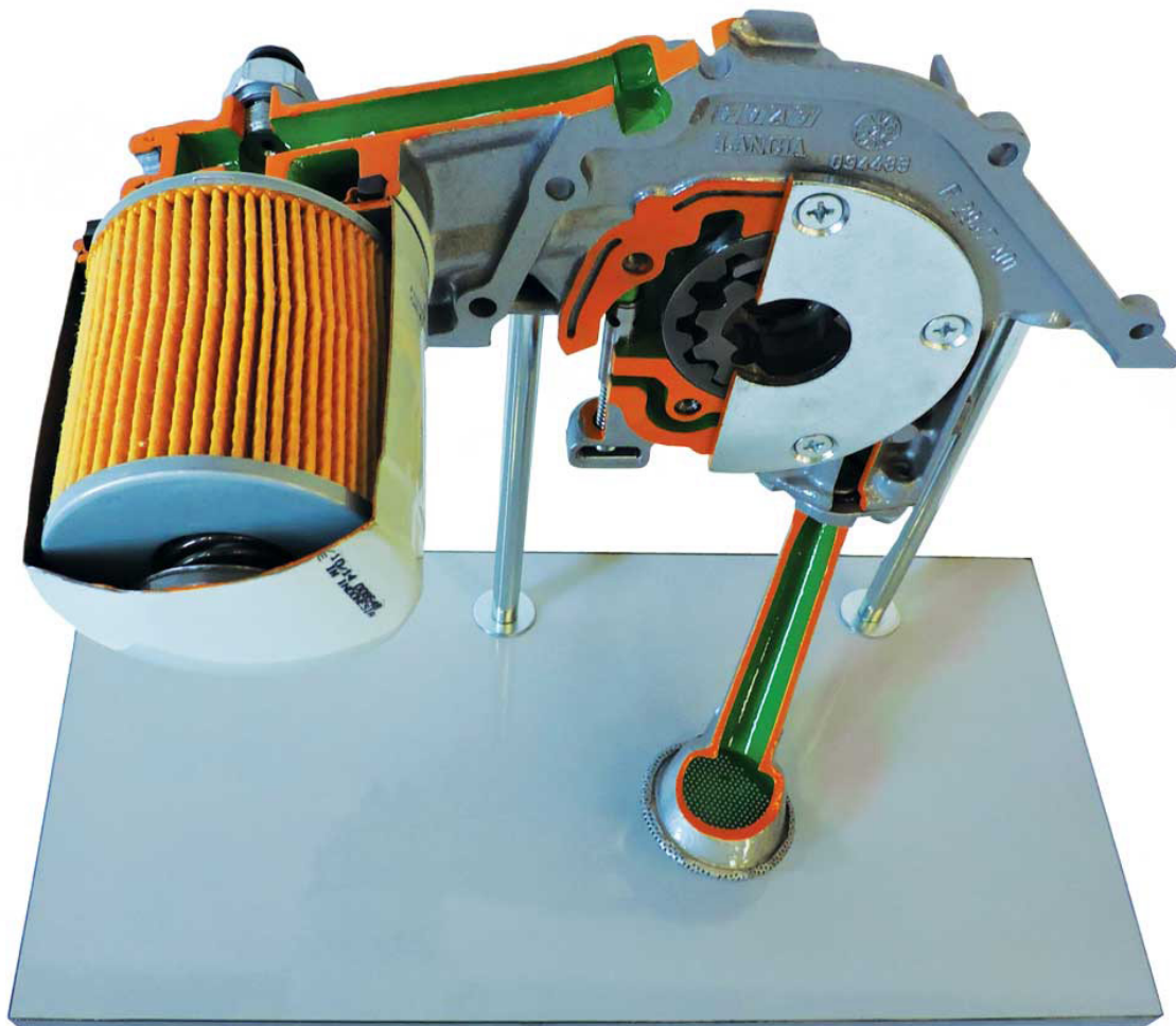
This product is a model of a Lubricating Circuit with Gear Rotor Oil Pump. It is mounted on a base.
